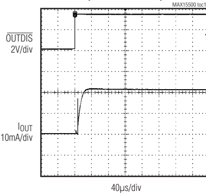
WAKEUP FROM STANDBY (CURRENT MODE)
